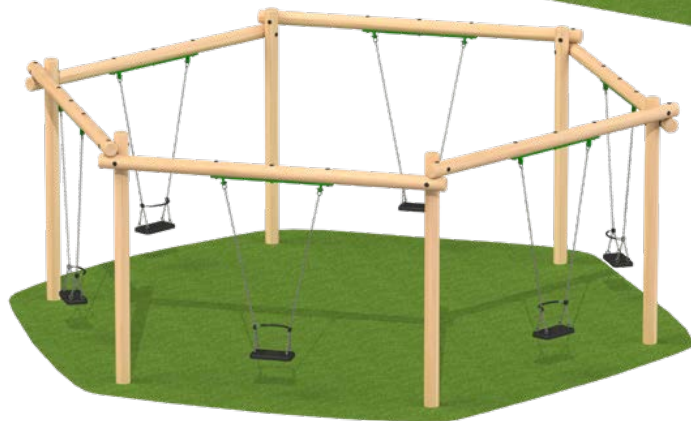
Six Seat Hexagonal Swing Frame Size: L: 7.04 W: 6.39 H: 2.62m Min space required: 13.12 x 12.24m Min Surface Area: 13.1 x 12.2m (60.9m 2 ) Free Fall Height: 1.4m
